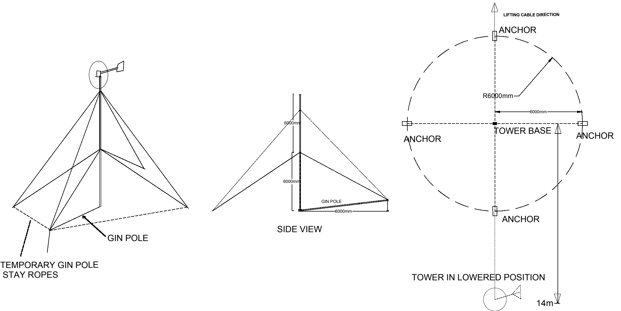
African Windpower 12 Meter Tower - Dimensions
